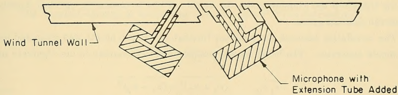
Figure 2 – Schematic of Microphone Adapted for Cross Spectral and Correlation Measurements
